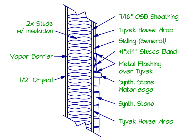
SIDING TO STONE DETAIL
