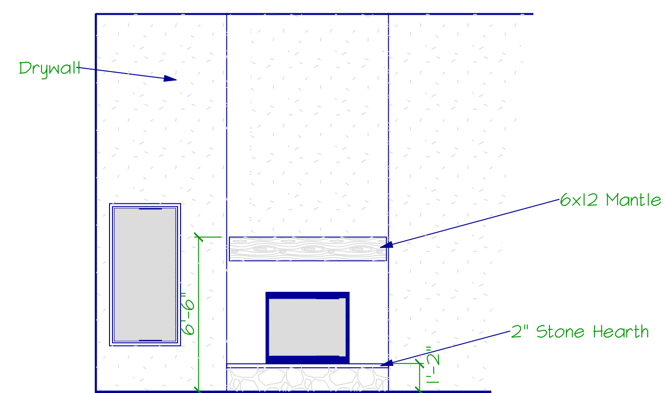
DETAIL A Scale 3/16" = 1'-0"
