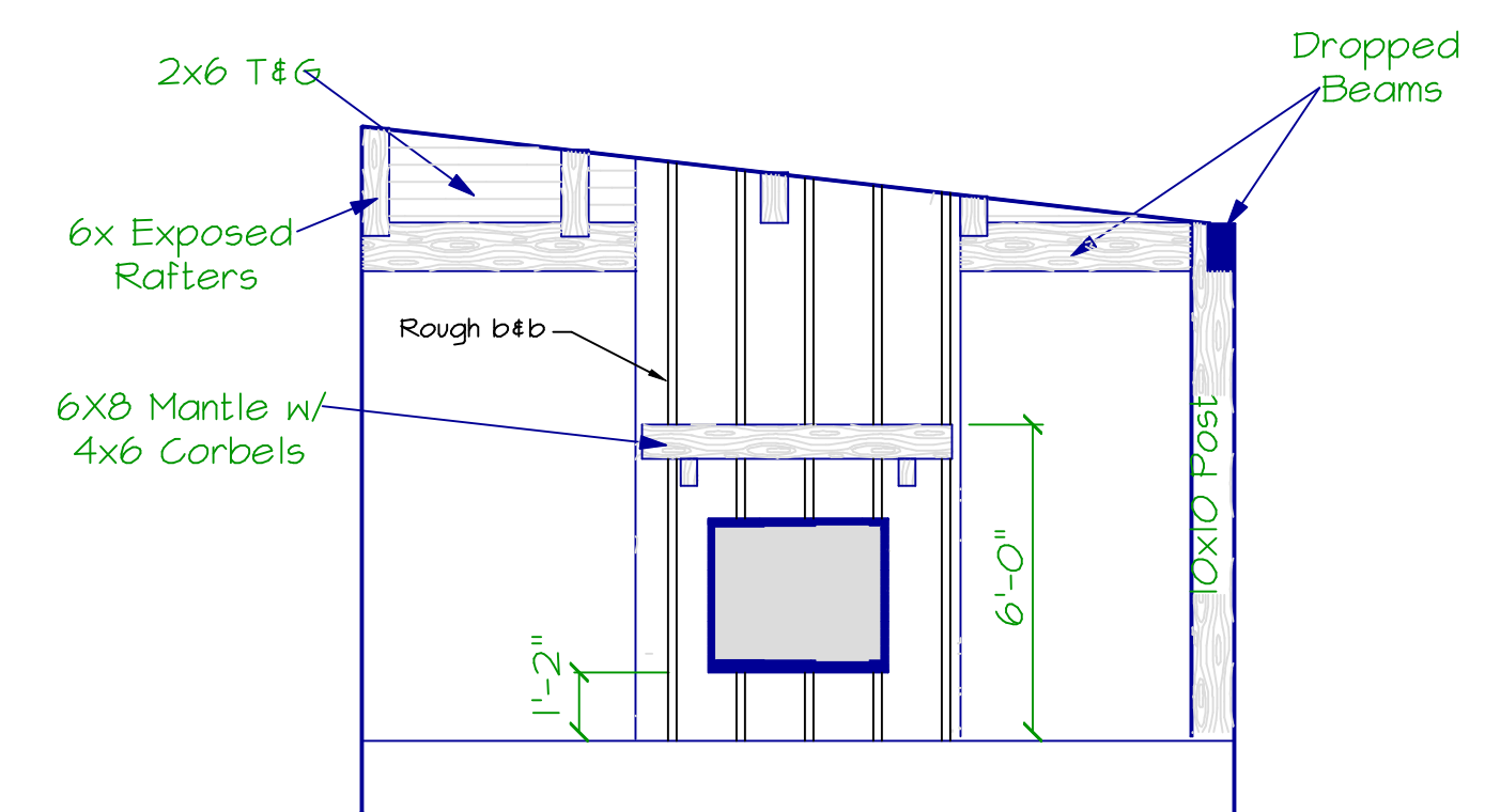
DETAIL B Scale 3/16" = 1'-0"
