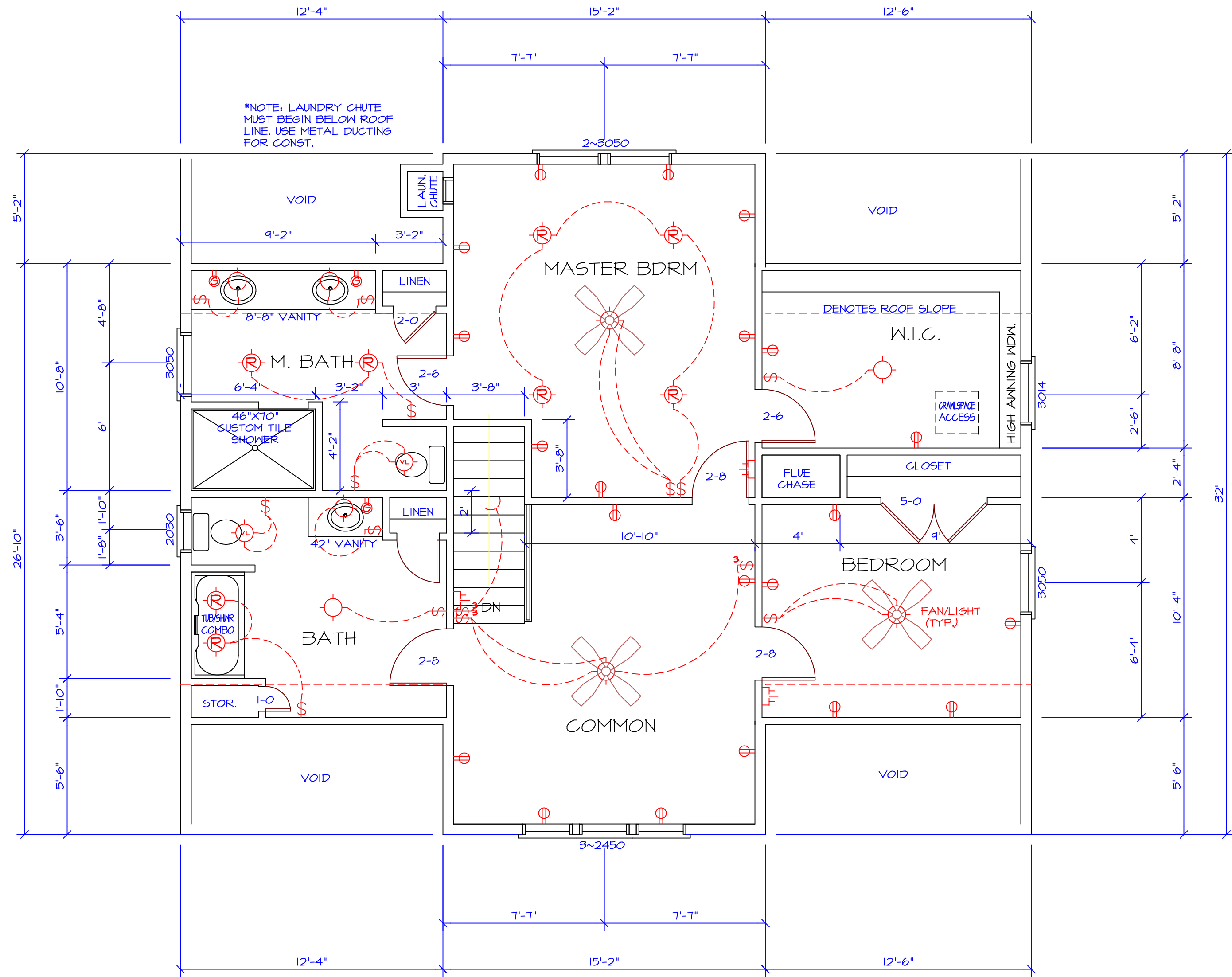
SECOND FLOOR PLAN SCALE: 1/4" = 1' - 0" 8' CEILINGSS
