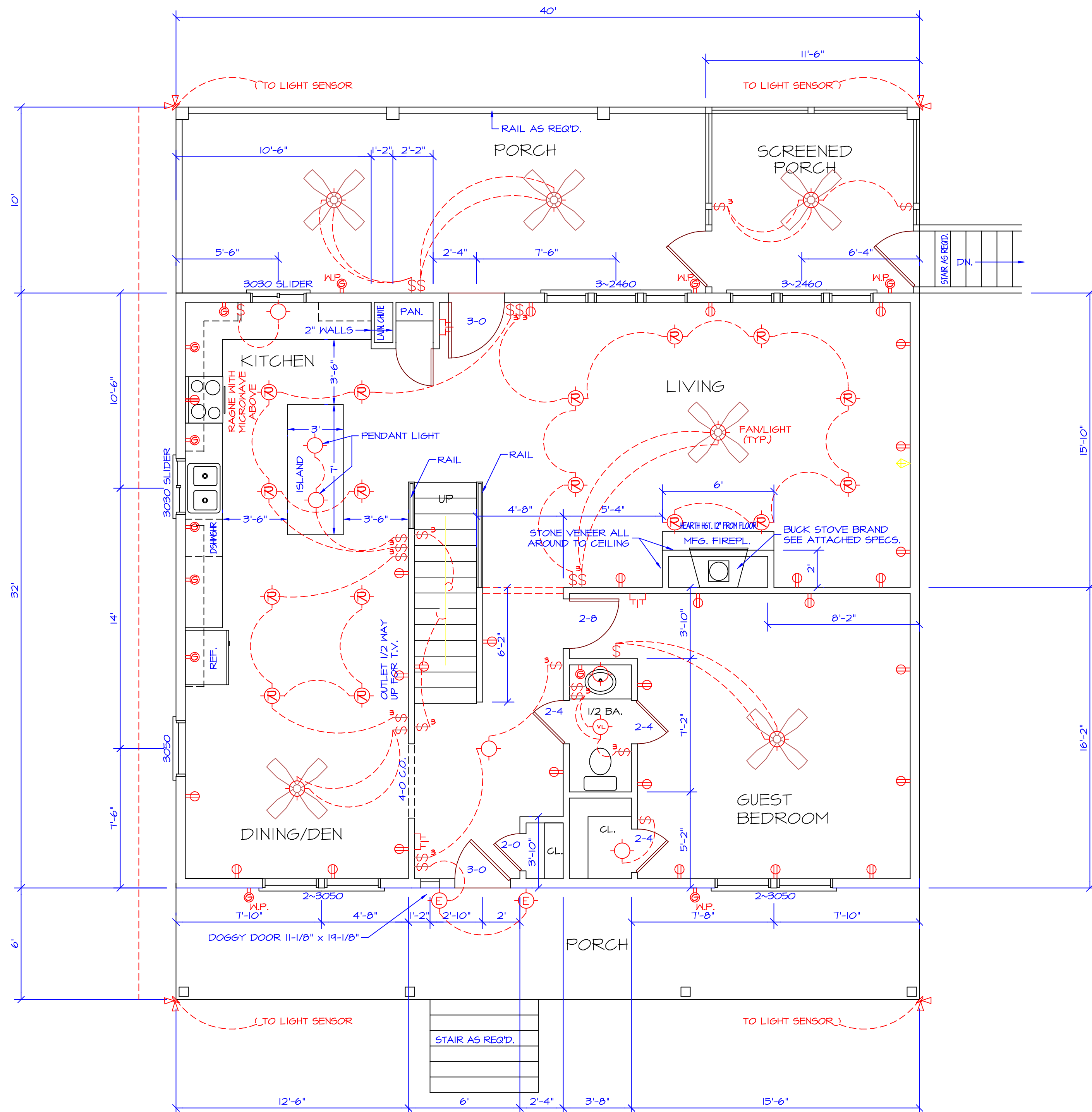
FIRST FLOOR PLAN SCALE: 1/4" = 1' - 0" 9' CEILINGSS
